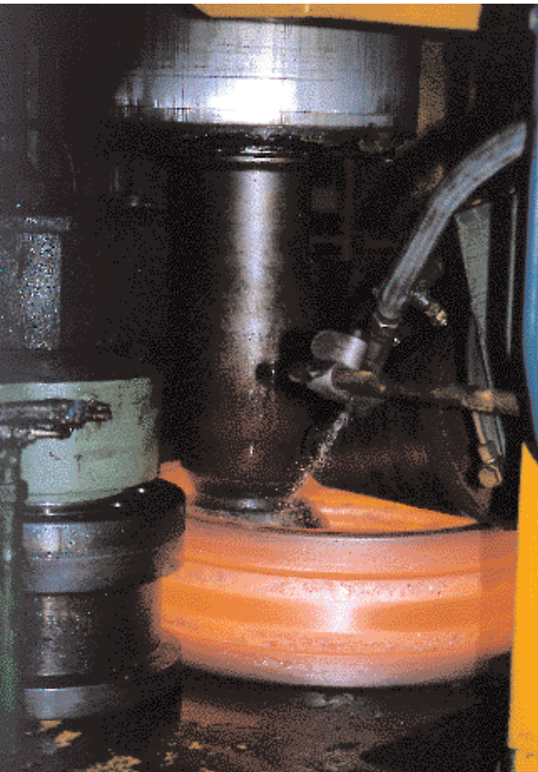
Ring rolling of tread rims
