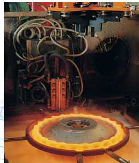
Single Shot Induction hardening
